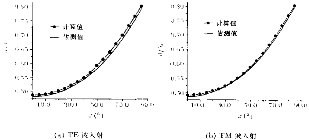
图 6 第一次强烈反射频率随水平入射角度的变化曲线 ( \epsilon_x = \epsilon_y = \epsilon_0 = 1.0, \epsilon_1 = 1.44, \epsilon_2 = 2.56, t_u/d = 2.037, t_f/d = 0.0, d_1/d = d_2/d = 0.5, \theta = 45^\circ )
