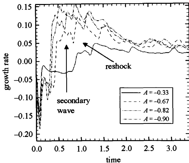
Fig. 9 Variation of perturbation growth rate vs. time at different Atwood numbers
