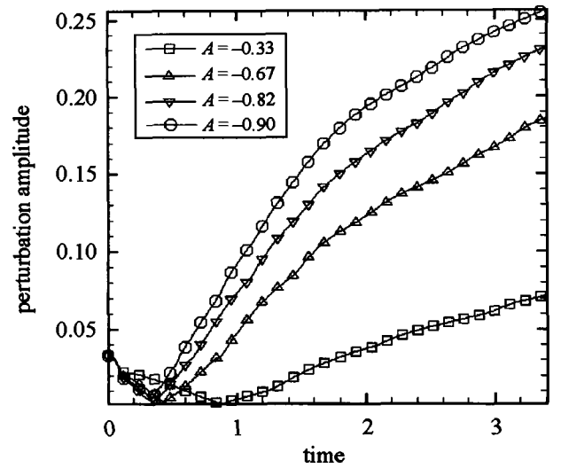
Fig. 7 Variation of perturbation amplitude vs. time at different Atwood numbers
