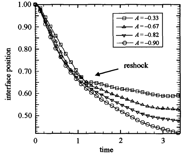
Fig. 8 Variation of averaged interface position vs. time at different Atwood numbers
