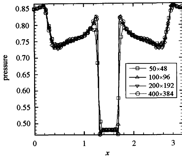
Fig. 1 Pressure distribution with different grids along a radial direction of 45^\circ and its mirror reflection part, where the circular center is located at x = 1.5
